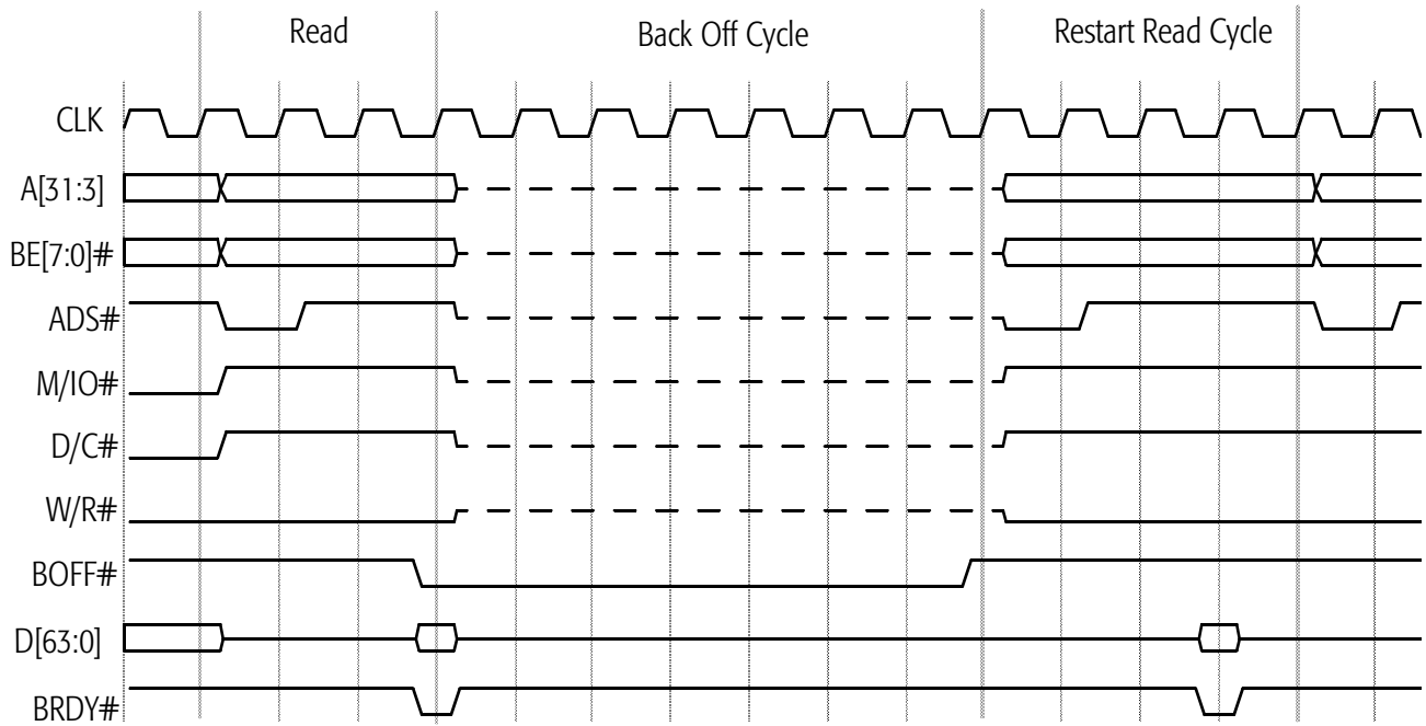
Figure 68. BOFF# Timing
